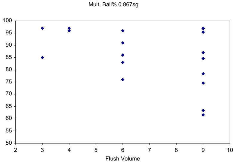
Graph 5. showing the number of plastic test balls (as a percentage) cleared from the pan with a full flush for a number of WCs at their design flush volume. Data from student experiments at Brunel and Heriot Watt, 1980–2002, courtesy of Professor John Swaffield.
