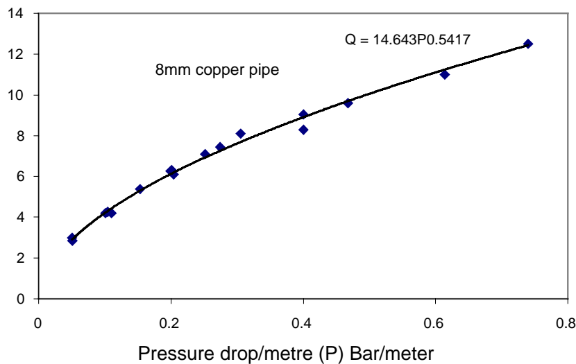
Graph 6. Results of tests to develop sizing charts for small bore pipe (Elemental Solutions).
