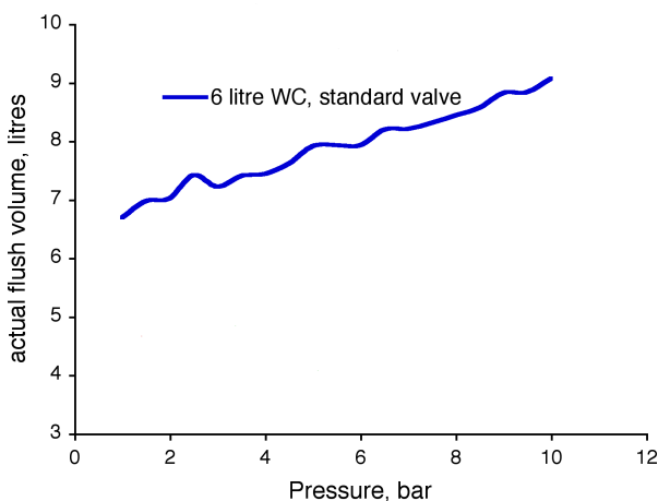
Graph 4. indicating flush volume against supply pressure for a nominally 6 litre WC. A delayed action inlet valve will maintain the nominal volume at all pressures. Data from WRc for 7.5 litre WC, scaled for 6 litre.
